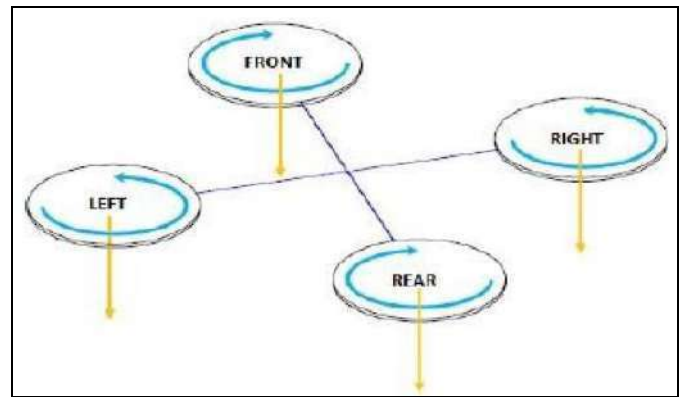
Fig.3.2. f Landing Motion of Quadcopter.
