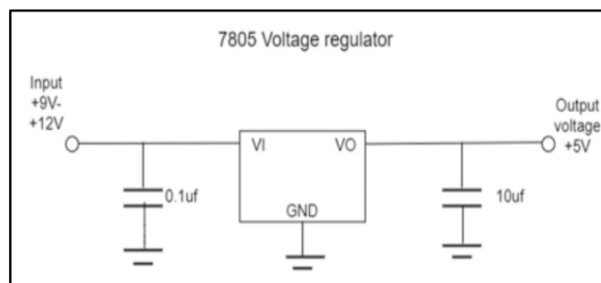
Fig. 2: 7805 Voltage Regulator
