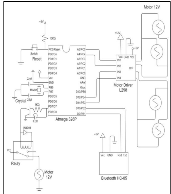
Fig.3: Circuit diagram of Android-based smart floor cleaning and sanitizing system
