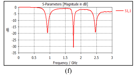
Fig. 2: Design steps with its reflection coefficient results at each stage. (a) Antenna design for 900 MHz. (b) S Parameter for antenna design in fig. 2(a). (c) Antenna design for 900 MHz and 1.8 GHz. (d) S Parameter for antenna design in fig. 2(c). (e) Antenna design for 900 MHz, 1.8 GHz and 2.4 GHz. (f) S Parameter for antenna design in fig. 2(e).
