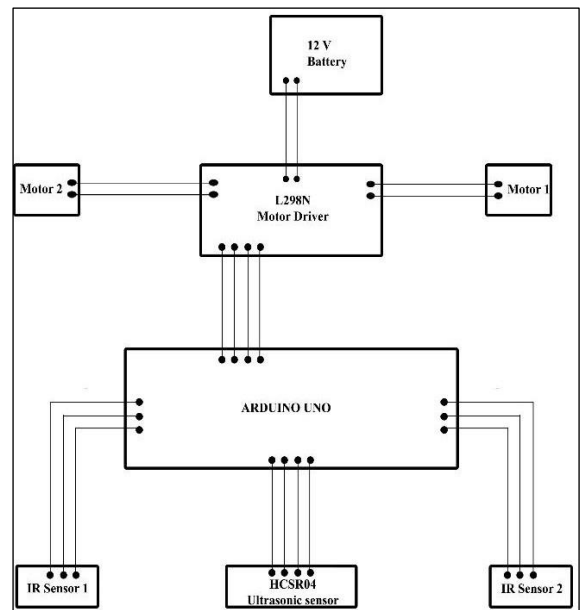
Figure 1. Overall Block Diagram
