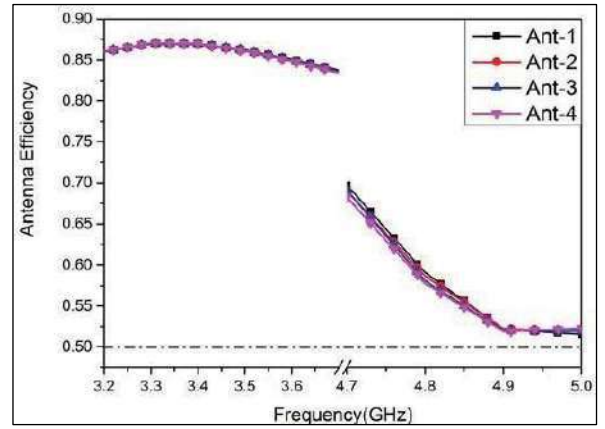
Fig. 4. Simulated Antenna Efficiency
