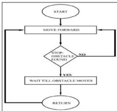
Fig.2.5.1: Algorithm steps
