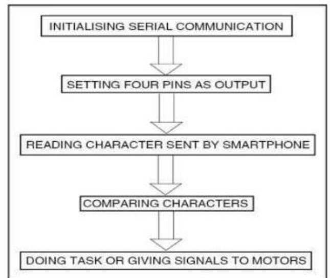
Fig 5.1. Flowchart
