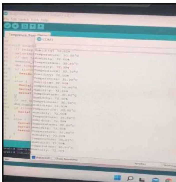
Fig 1.9 Program Code
