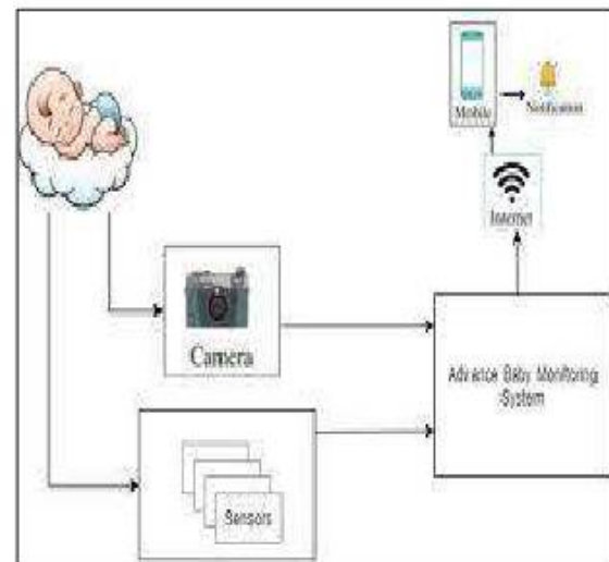
Figure 1: Workflow
