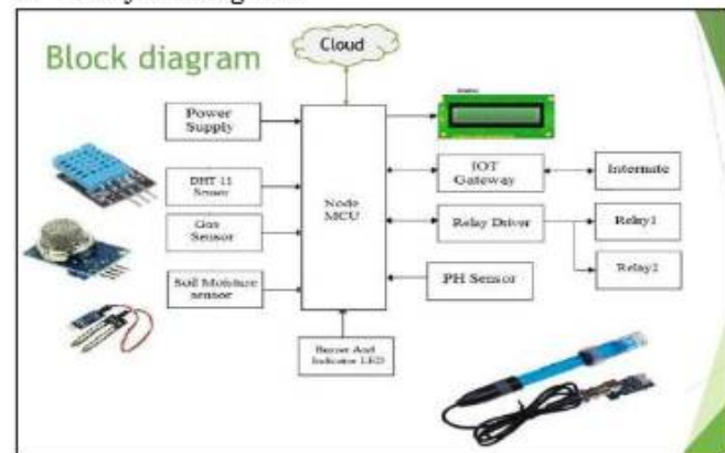
Fig 3.1: Block Diagram
