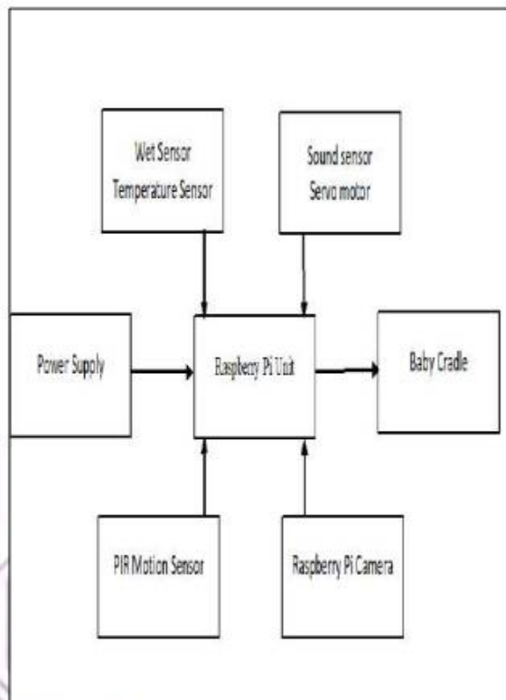
Figure 2: Block Diagram
