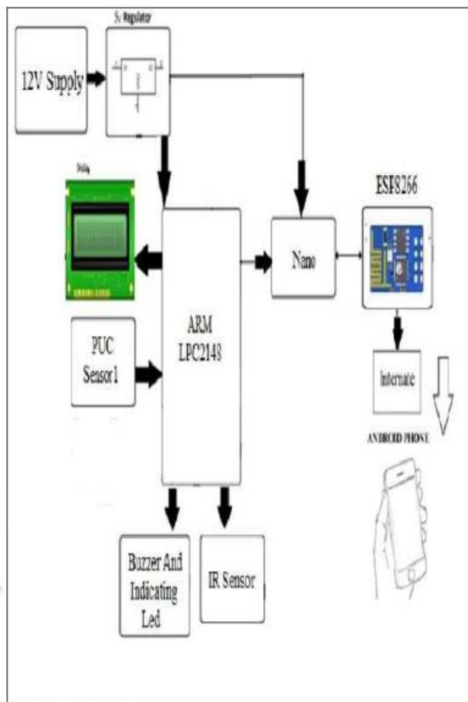
Fig 1. Block Diagram
