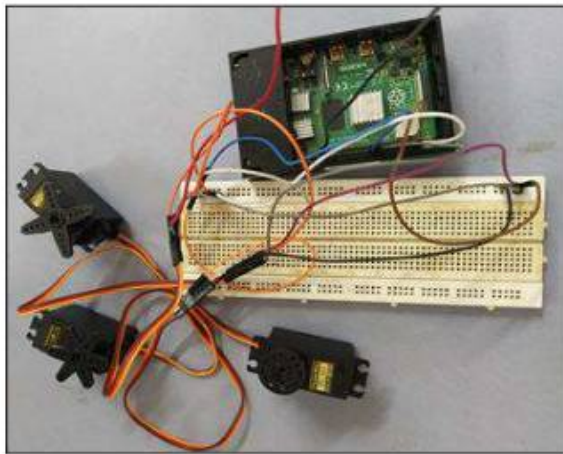
Fig 4.3 servo motors connection
