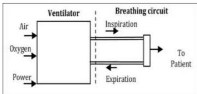
Fig 1.1: Schematic of Mechanical Ventilator
