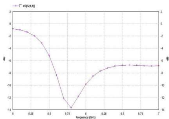
Fig.9. Return loss of 3X3 SPPA
