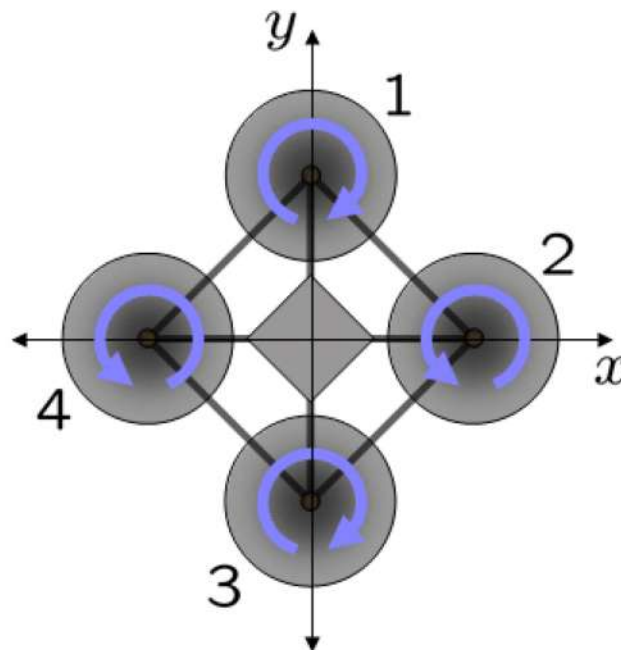
Fig. 3. Motion of Quadcopter
