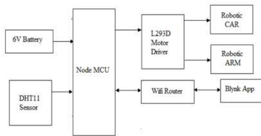
Fig.1. Block Diagram of System
