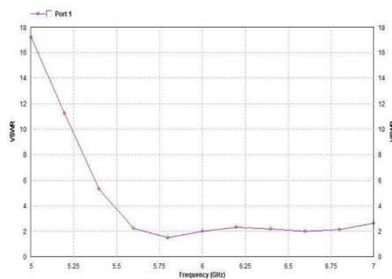
Fig.15. VSWR versus frequency graph of 4X4 SPPA
