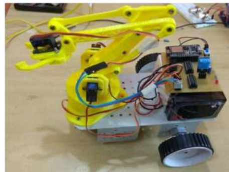
Fig.8. Automation model
