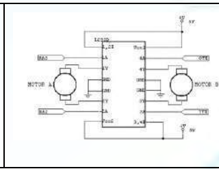
Fig 3.4.: L293D with DC motor Pin Diagram
