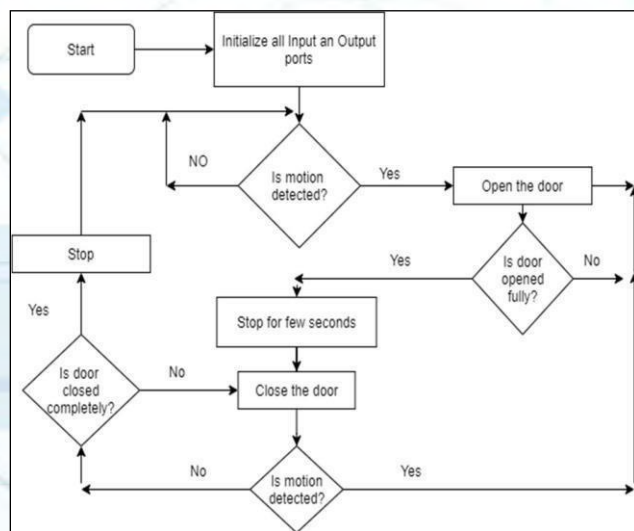
Figure.3. Flowchart of Automatic Door Opening System with Entry Counter
