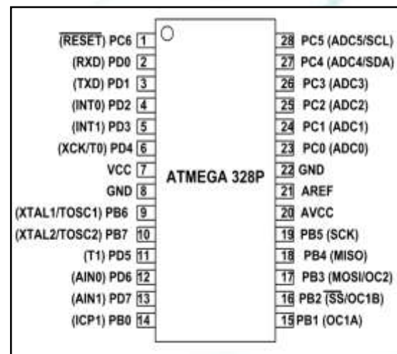
Figure 2.1 ATMEGA 328P Pin Configuration
