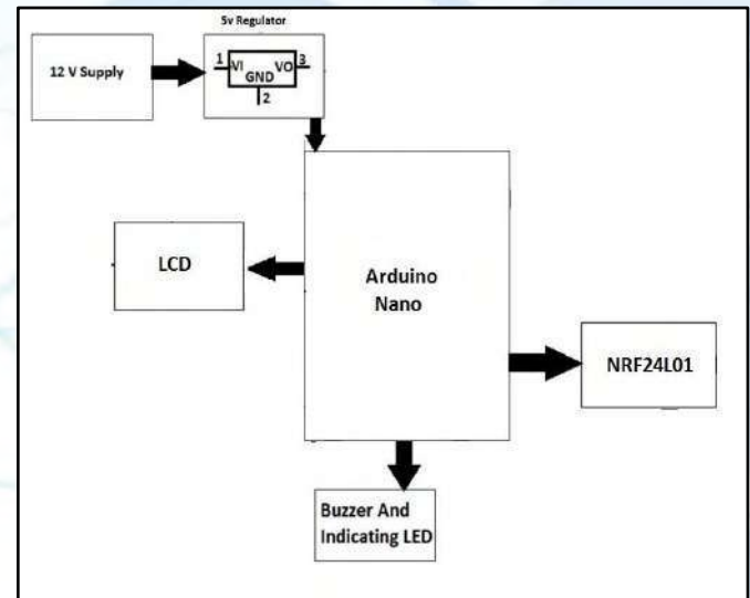
Fig 2: Receiver Block Diagram
