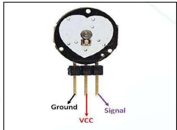
Fig. 4: Pulse sensor
