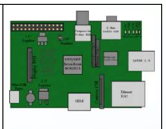
Fig 3.2.: Raspberry Pi
