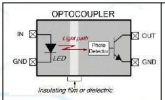
Fig 3.5: Optocoupler
