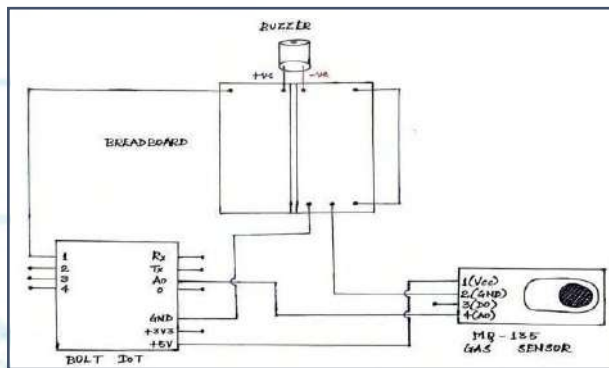
Figure 2 Circuit diagram
