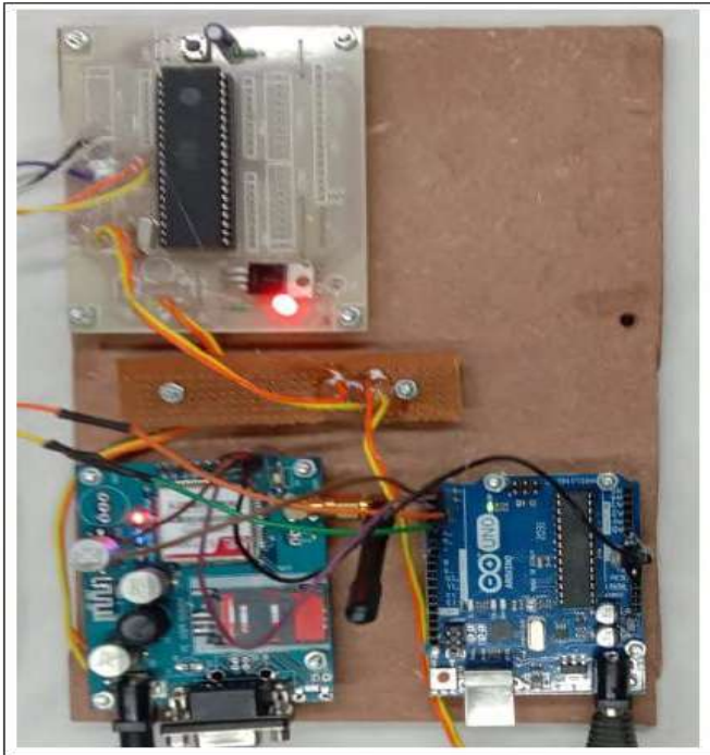
Fig 4. Microcontroller 8051 Interfaced with Arduino UNO + GSM module
