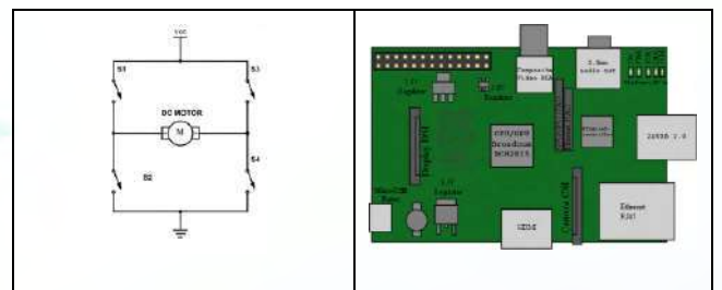
Fig 3.1.: H-Bridge Structure
