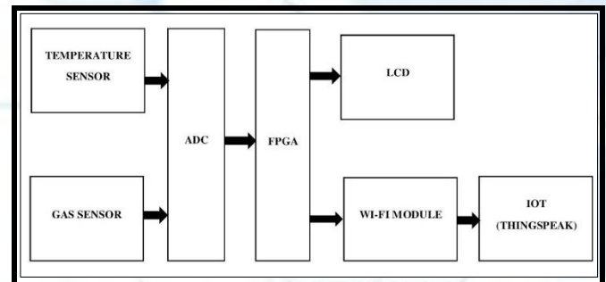
Fig.1 Overview of the gas leakage detection system
