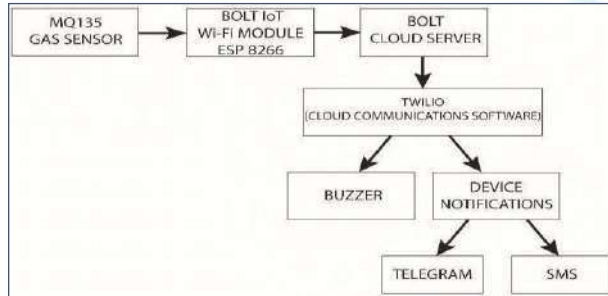
Figure 1 Activity Diagram
