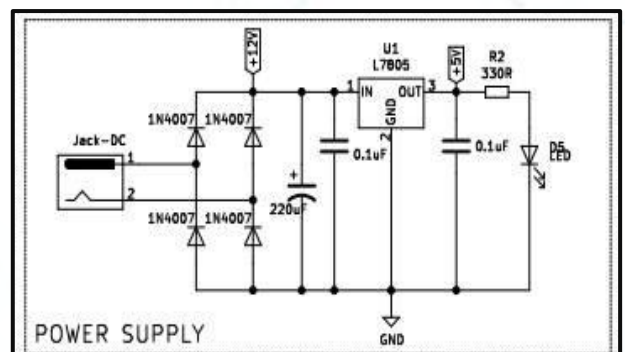
Fig. 6 Power supply of 12v
