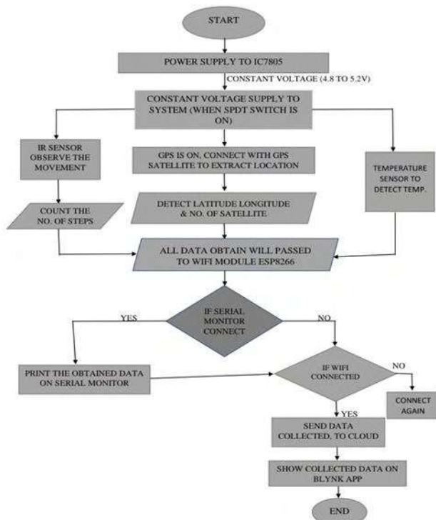
Fig. b Flowchart of working system
