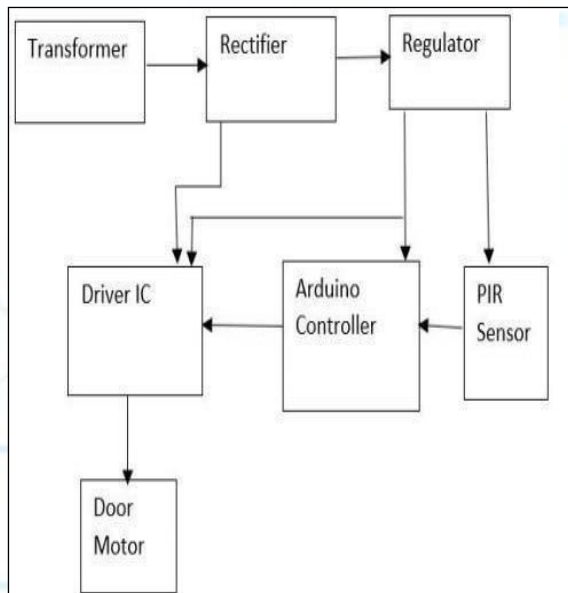
Fig.2. Block Diagram
