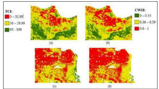
Figure 2.2: The Results of TCI and CWSI | Source: [2]
