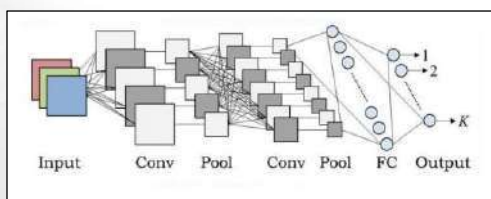
Fig 3.2. CNN architecture
