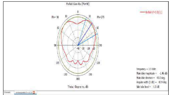
Fig. 3.9 Polar plot
