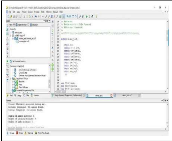
Fig.6: Code Output
