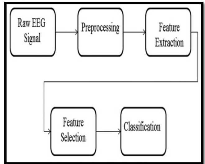
Fig 3. Classification Steps
