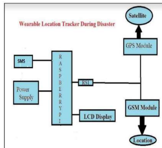
Fig 3.4 Block Diagram
