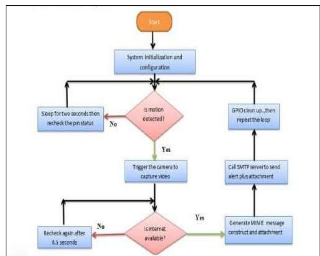
Fig 3.1: Flow Chart Implementation
