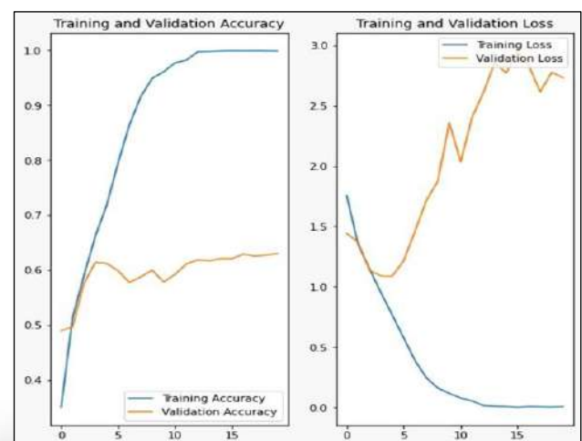
Fig 4.3. The below is an accuracy X epoch graph because of overfitting.
