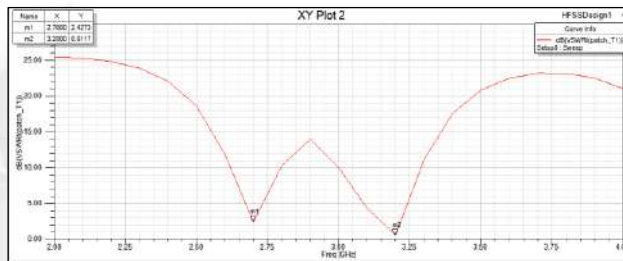
Fig 5.3: VSWR
