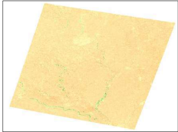
Figure 5.5: NDVI of Rosebud Region for Year 2019
