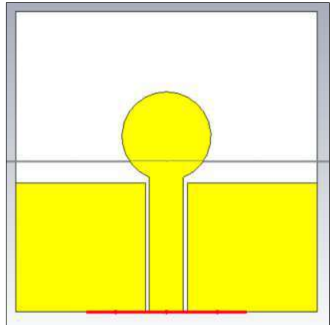
Fig 3. Circular Patch Monopole Antenna
