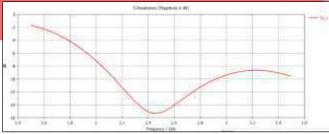
Fig 4. S 1,1 Graph of circular patch antenna
